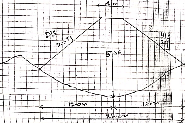
X-SECTION AT RD 20
