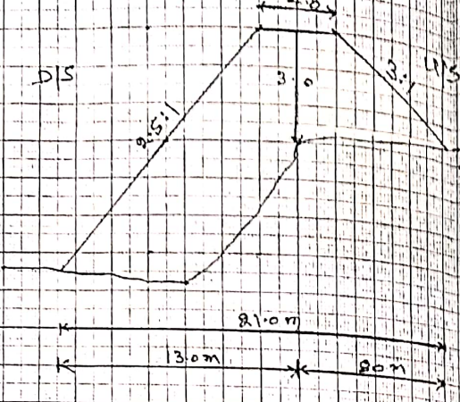
X-SECTION AT RD 10
