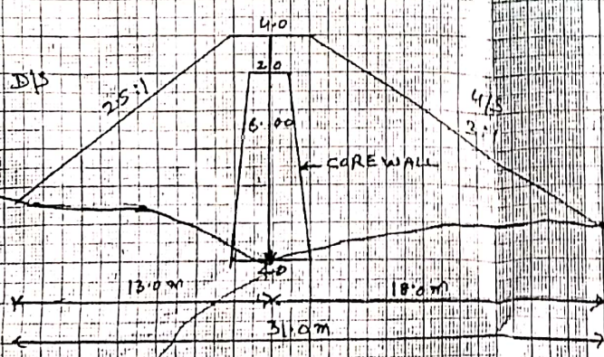
X-SECTION AT 25
