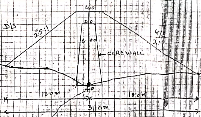
X-SECTION AT 25
